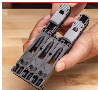
Positioning sliders for 1/2" and 3/4"-thick materials
