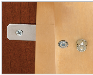
Adjustable door-mount brackets (US Patent No: 8,388,076) and jack screw for precise door alignment
